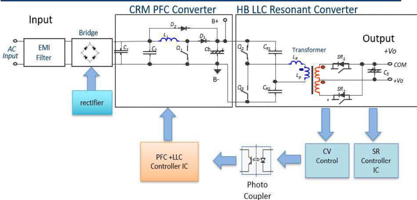
Note: Block Diagram for CRM PFC + HB-LLC
