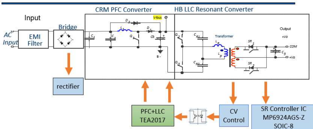
Note: Block Diagram for CRM PFC + HB-LLC
